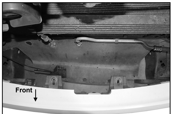
(Fig 4) Remove hood latch bracket from back of bumper
