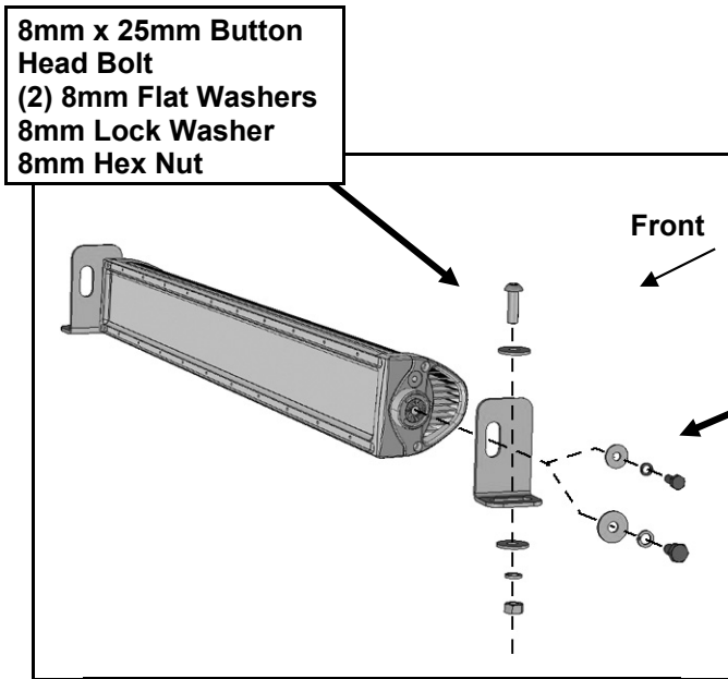
(Fig 12) Attach LED bar style light to "L" Brackets (light available separately)
