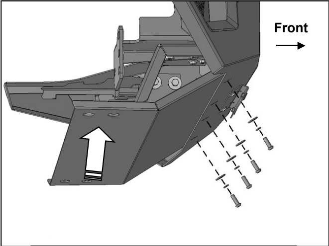
(Fig 2) Line up back mounting holes on Skid Plate (arrow) with holes in Support Bracket and frame for tow hook
