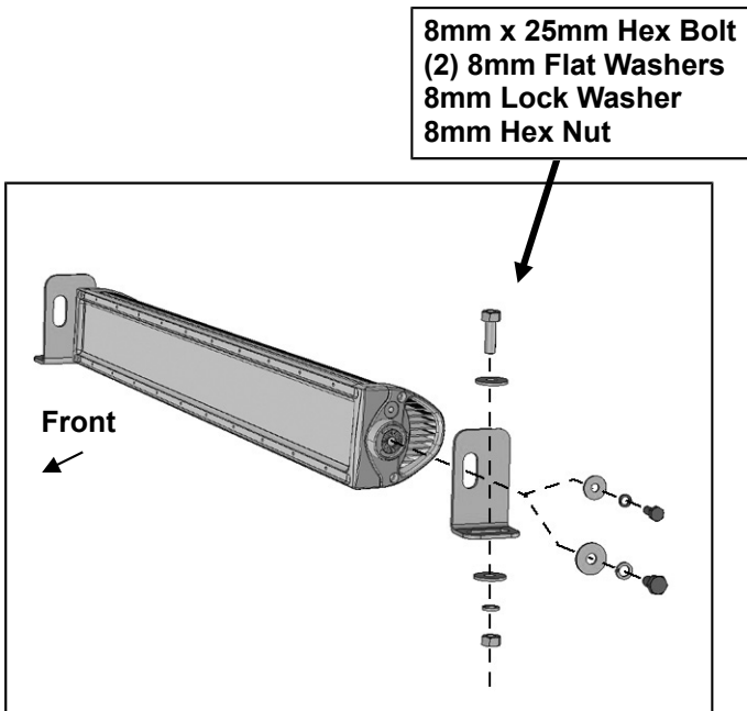
(Fig 12) Bracket illustration is a suggestion only. Brackets are offset to allow adjustment for all widths of lights
