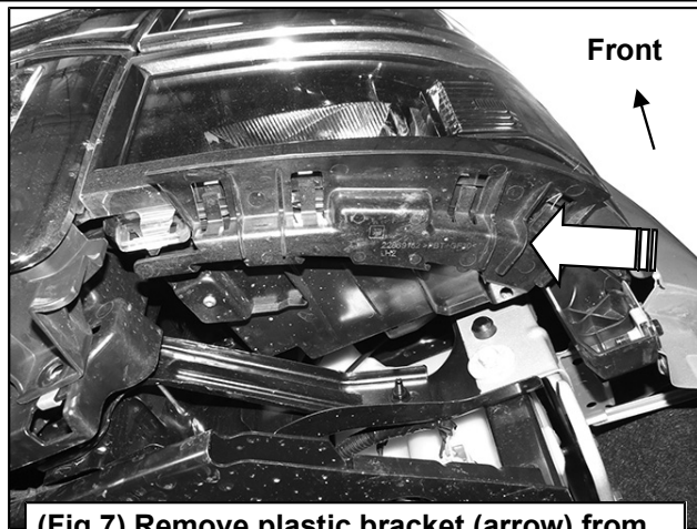
(Fig 7) Remove plastic bracket (arrow) from bottom of headlight (driver/left side pictured)
