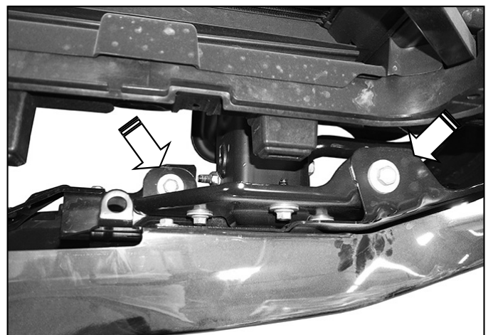
(Fig 4) Remove bumper bolts (pictured from above)
