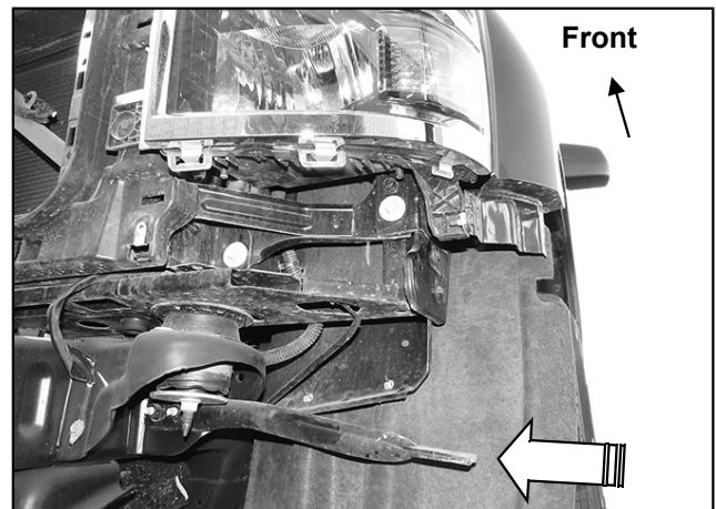
(Fig 8) Remove outer bumper supports (arrow)
