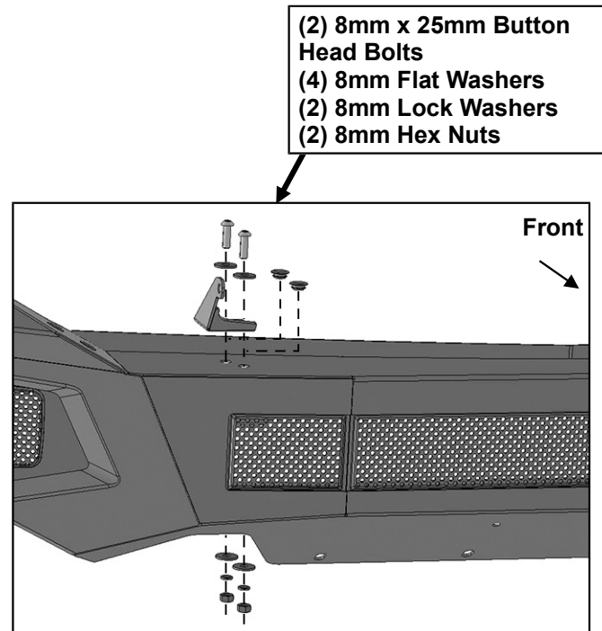
(Fig 13) Remove rubber plugs to attach Top Light Bracket to Bumper
