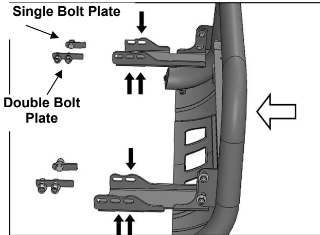
(Fig 13) Typical Silverado/Sierra mounting position
