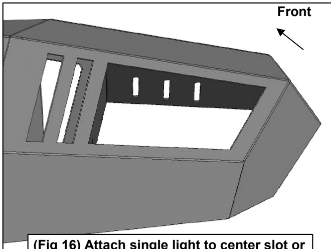
(Fig 16) Attach single light to center slot or use inner and outer slots for dual lights
