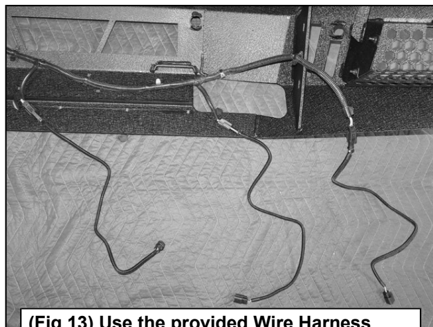
(Fig 13) Use the provided Wire Harness extensions for the Passenger side sensors
