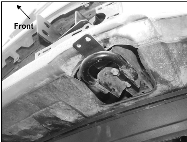
(Fig 7) Brackets installed, model with tow hook pictured
