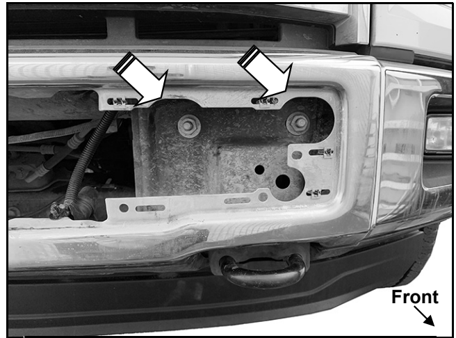
(Fig 2) Remove (2) factory hex nuts (arrows)
