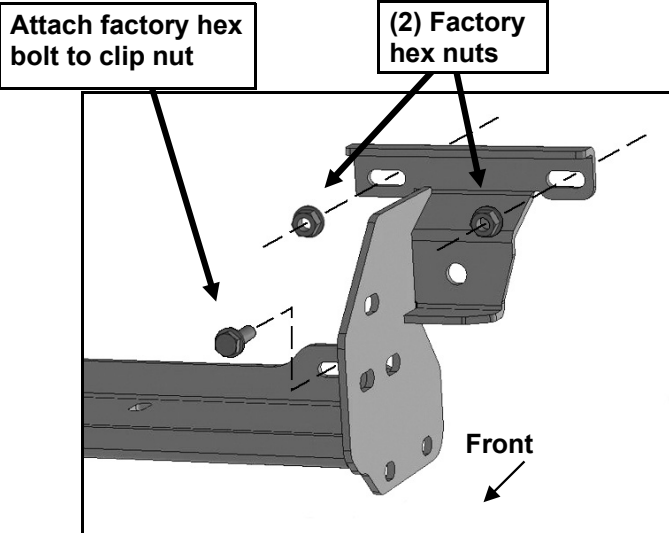
(Fig 11) Reuse factory hardware to attach Winch tray/Bracket assembly to factory bumper brackets (driver/left side pictured)
