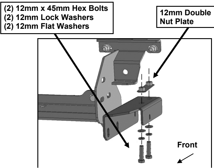
(Fig 13) Attach driver/left Frame Support Bracket to double nut plate in frame channel
