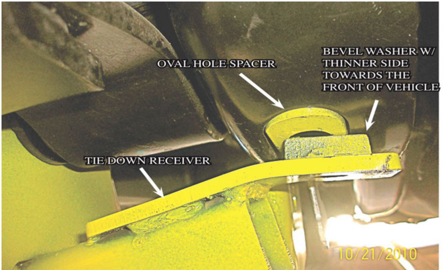
PHOTO F) LOOKING UP FROM UNDER THE SPRING PERCH
