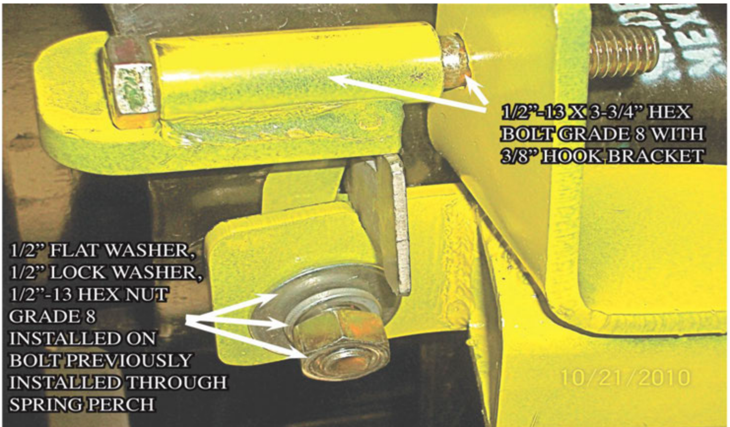
PHOTO F) LOOKING UP FROM UNDER THE SPRING PERCH
