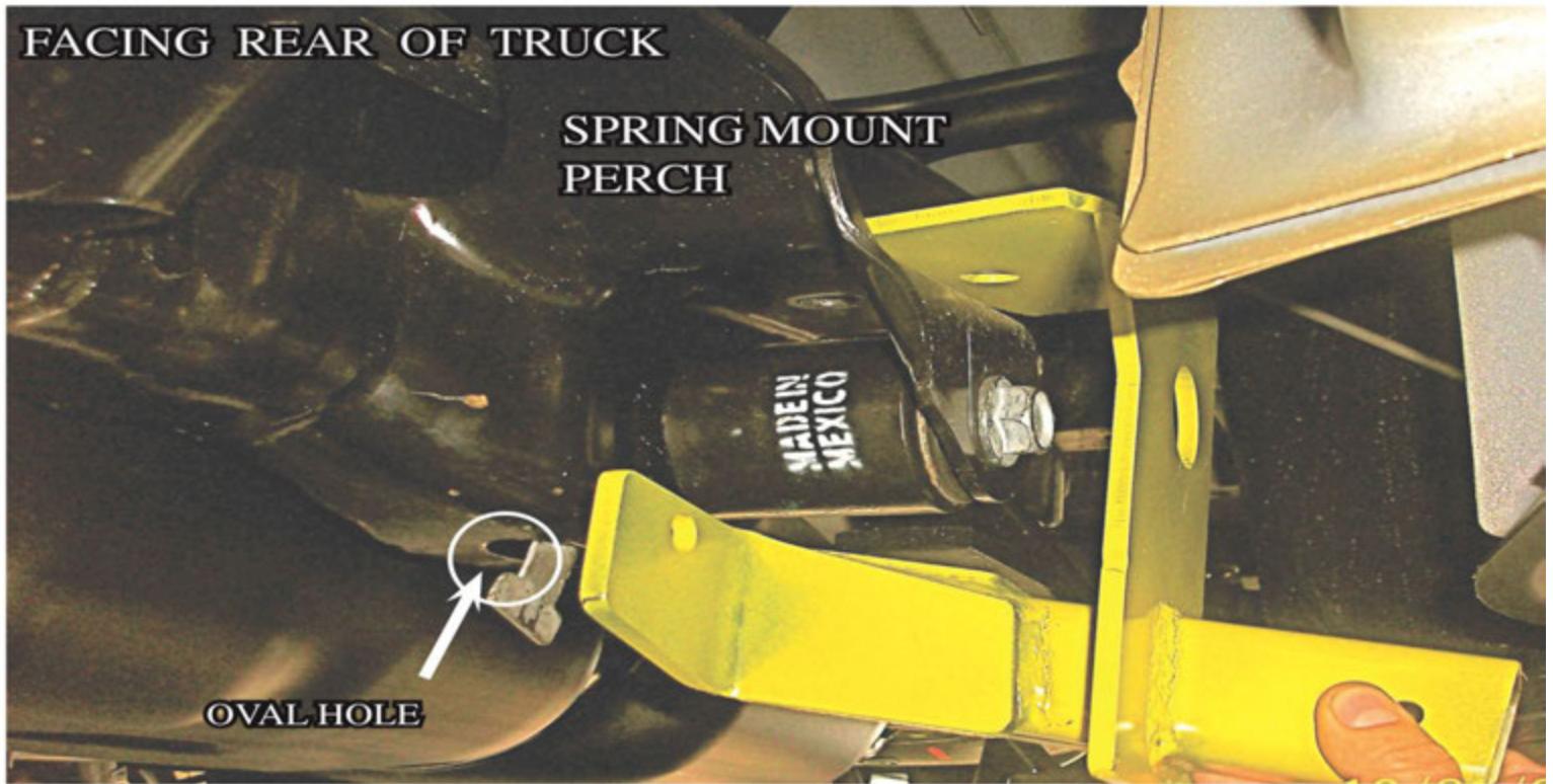
PHOTO C) TOP OF PLATE
