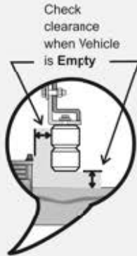
Typical Light Duty Installation
