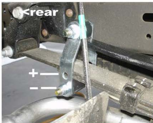
adjust pre-load & ride height
