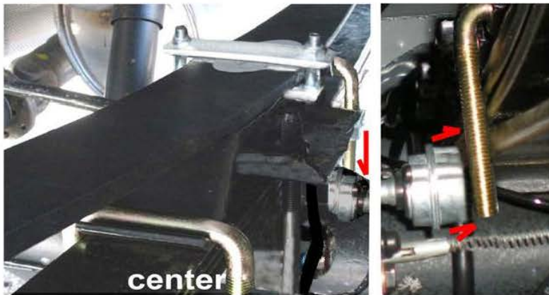
center install hardware clear of factory sensor at axle rear
