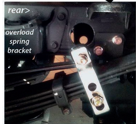
SSA16 installed heavily loaded
