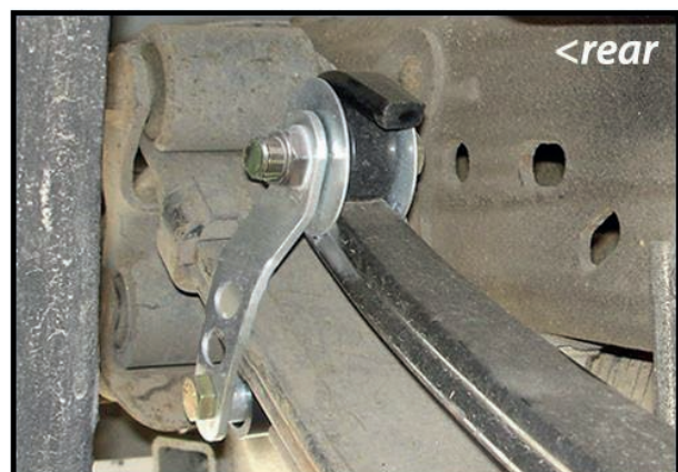
Adjustable pre-load and ride height [frnt/rear]
