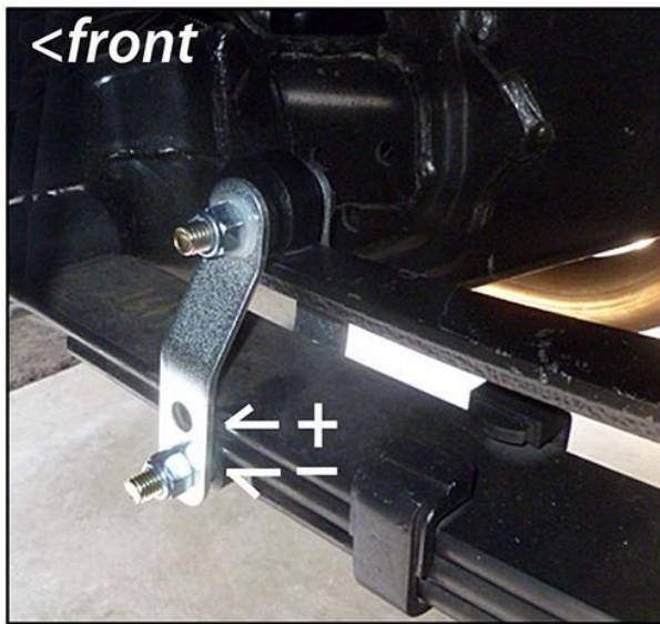
SuperSprings Mounting Kit #MTKT Installed
