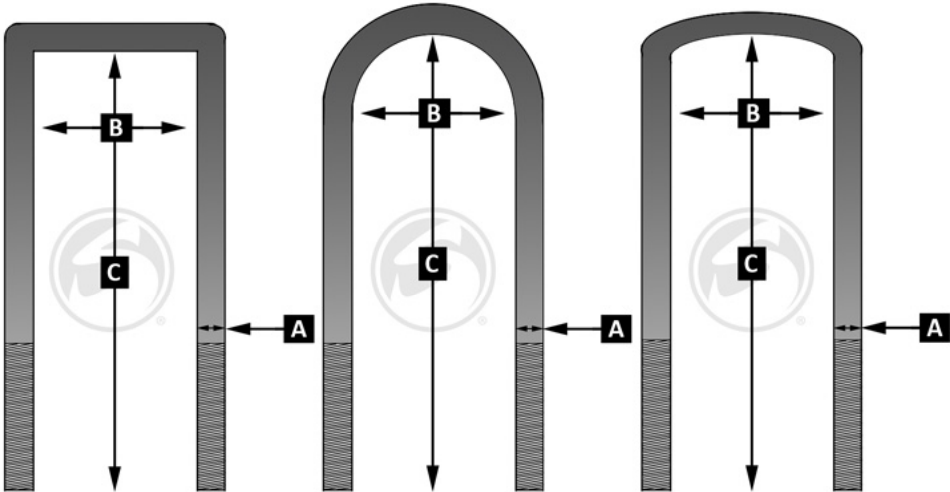
Square Bend
