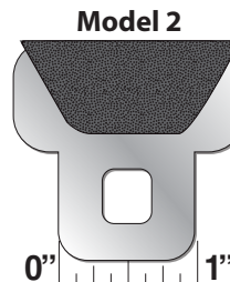
Model 2 10" Universal Seat Belt Extension 1" Locking Tab Width Webbing Construction 46-3102 - 1 per hanging card
