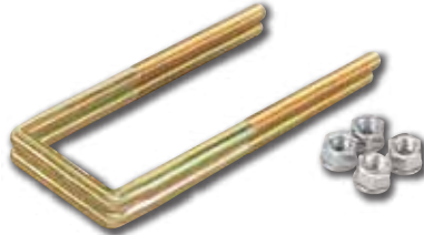
13-0190A - PAIR PACK - Square U-Bolt kit Contains: 2 Square U-Bolts 4 Nuts and 4 Lock Washers
