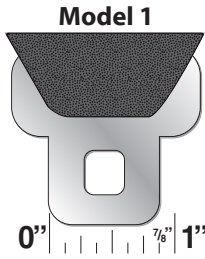
Model 1 7" Universal Seat Belt Extension 7/8" Locking Tab Width Webbing Construction
