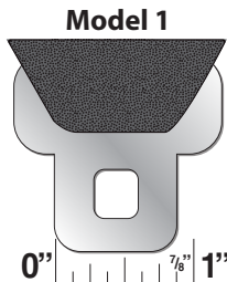
Model 1 7" Universal Seat Belt Extension 7/8" Locking Tab Width Webbing Construction 46-3371 - 1 per hanging card
