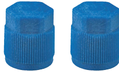
Part # 613-10 Low Side Blue R-134a 15 mm Fitting Service Port Cap, 9mm x 1
