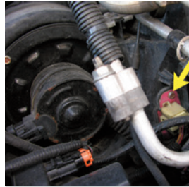
Remove Screw
