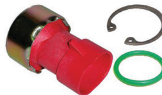
Part # 26746 Compressor Mounted High Cut-Out Pressure Switch GM Denso 10S - High Pressure Cut-Off (Red - Replaces Purple and Orange) Switching Pressure: 470 CADILLAC 2002-2007 CHEVROLET 1999-2009 GMC 1999-2009
