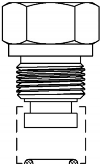
Swivel O-Ring Type II
