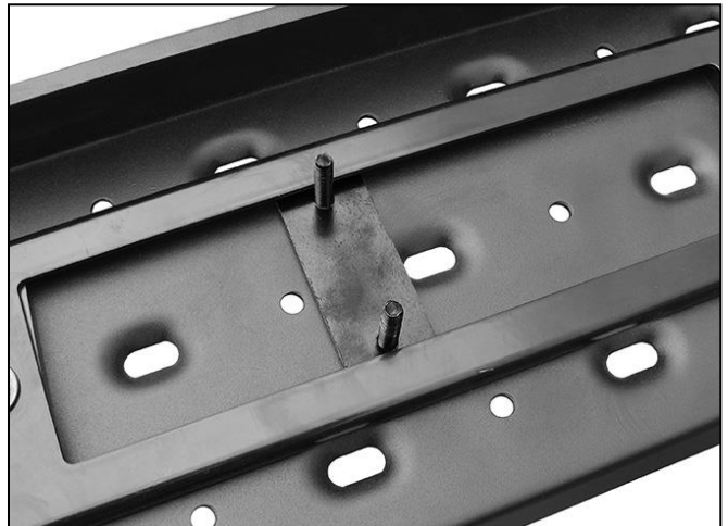
(Fig 12) Slide 6mm Double Bolt Plate into channels
