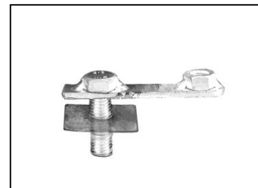
(Fig 2) 12mm Bolt-10mm Nut Plate w-Retainer, NOTE: 10mm hardware not required on models with threaded inserts
