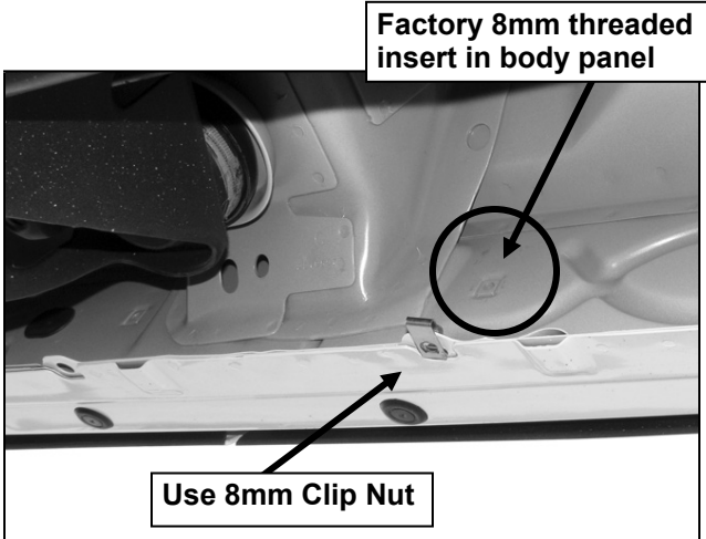
(Fig 3) Example of factory hole in flat mounting tab and threaded hole in body panel
