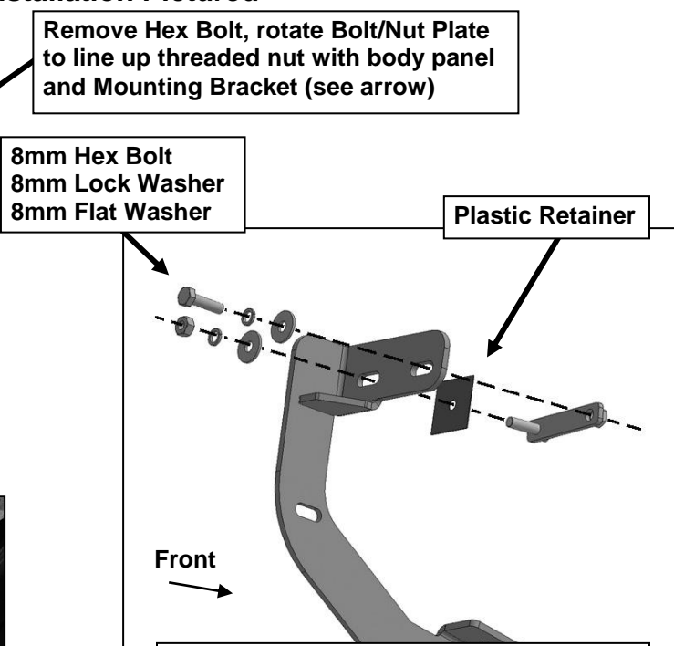
(Fig 6B) Attach Bracket to threaded end of Bolt Plate first. Remove 8mm Hex Bolt (see Fig 3). Rotate Bolt Plate to line up with remaining factory hex shaped hole.
