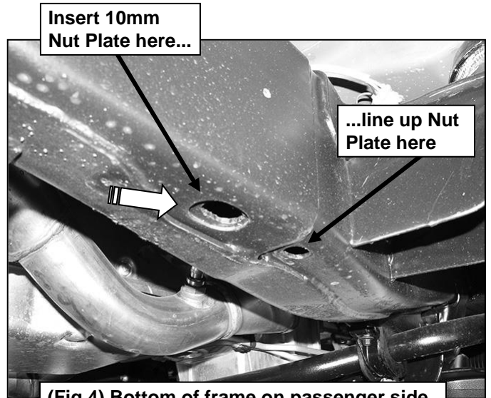
(Fig 4) Bottom of frame on passenger side
