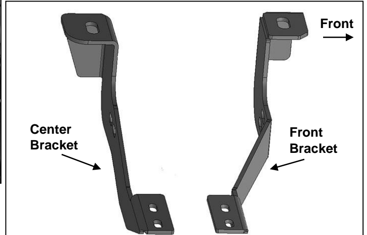
(Fig 2) Passenger side front and center Brackets
