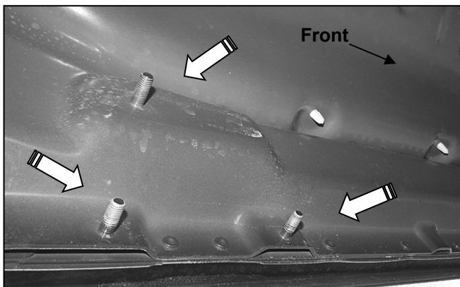
(Fig 1) Locate the (3) factory threaded studs at each location. Driver side rear pictured
