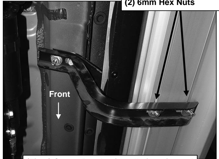
(Fig 6) Center Bracket installation pictured
