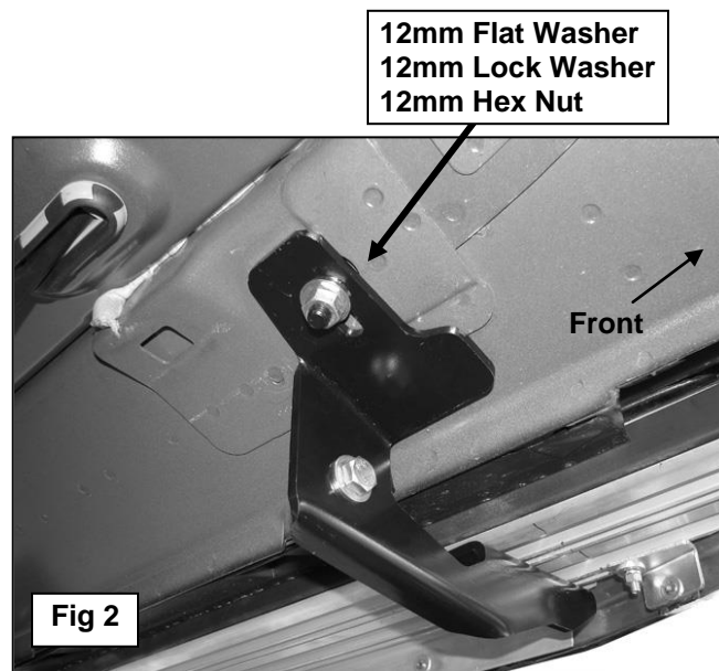
12mm x 35mm T-Bolt Plate 12mm Flat Washer 12mm Lock Washer 12mm Hex Nut
