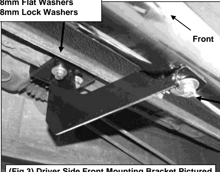
(Fig 3) Driver Side Front Mounting Bracket Pictured
