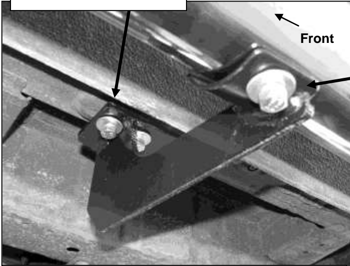
(Fig 4) Driver Side Center Mounting Bracket Pictured
