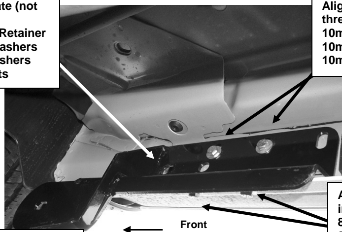
(Fig 3) Regular Cab passenger side Front Mounting Bracket pictured
