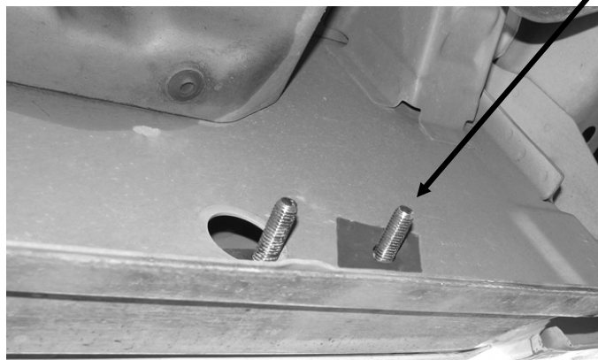
Fig 5 Super Cab passenger side rear mounting location pictured. Shown with Plastic Retainer in place
