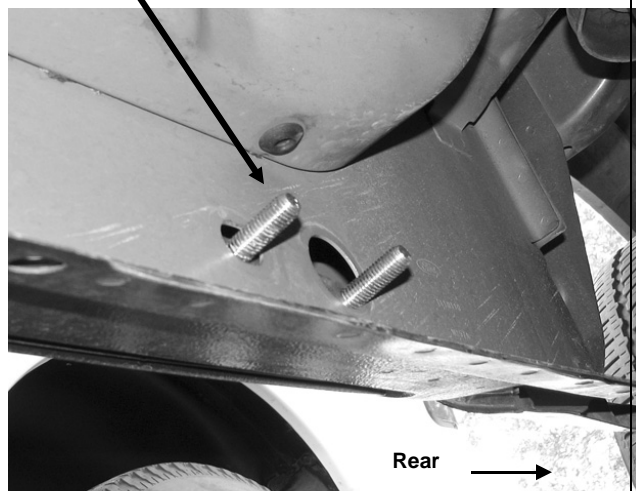
Fig 5 Regular Cab and Super Crew Cab passenger side rear mounting location pictured
