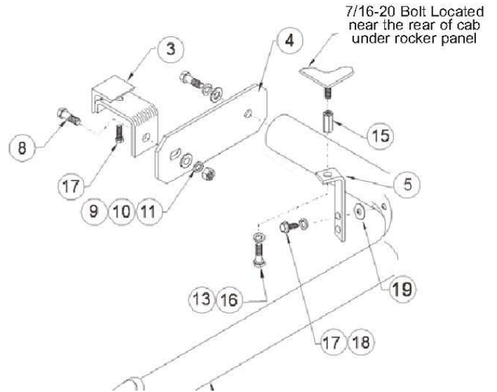
FIGURE 1 - DRIVER-FRONT
