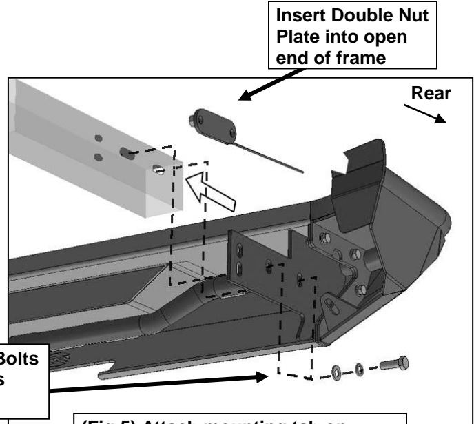
(Fig 5) Attach mounting tab on Bumper Center Section to Nut Plate
