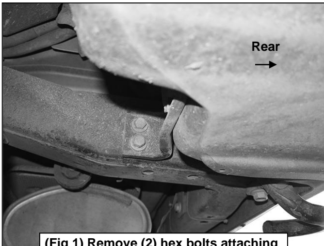
(Fig 1) Remove (2) hex bolts attaching support bracket to side of frame
