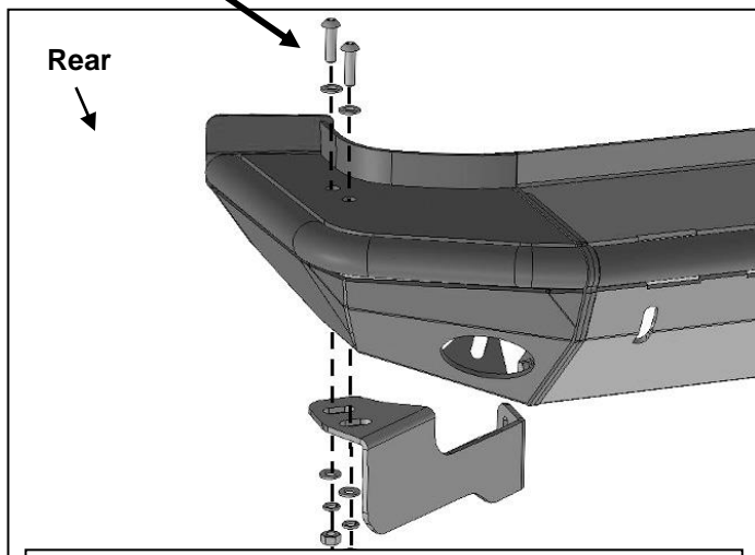
(Fig 6) Attach driver side Support Bracket to Wing
