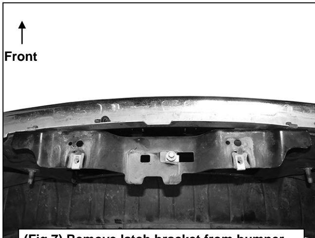
(Fig 7) Remove latch bracket from bumper
