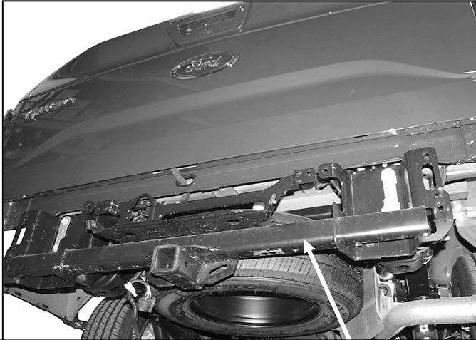
(Fig 13) Reinstall integrated receiver hitch/bracket assembly on models with "HD Towing" package
