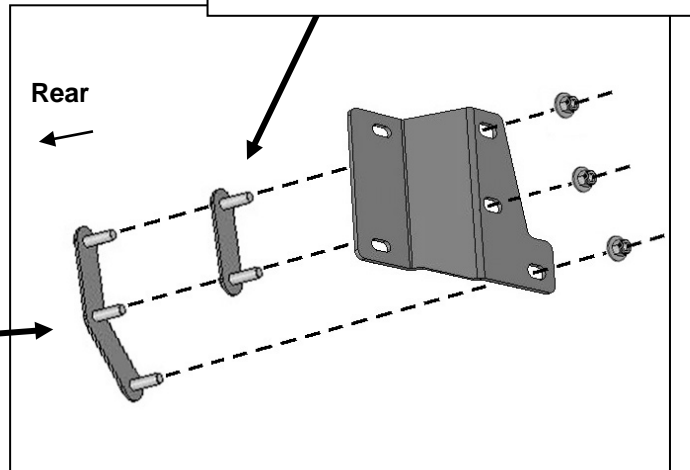
(Fig 10) Reuse either factory bolt plate to attach passenger/right Mounting Bracket to end of frame
