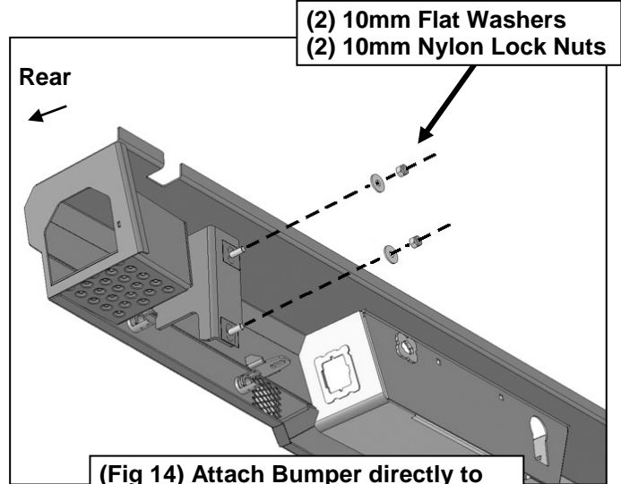
(Fig 14) Attach Bumper directly to integrated hitch bracket (see Fig 12)
