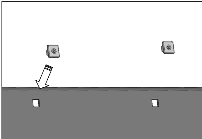
(Fig 15) Push plastic plugs into holes for license plate
