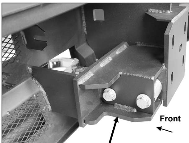
(Fig 9) Reuse factory hardware to attach tow hook to mounts in Bumper (passenger/right side pictured from back of Bumper)
