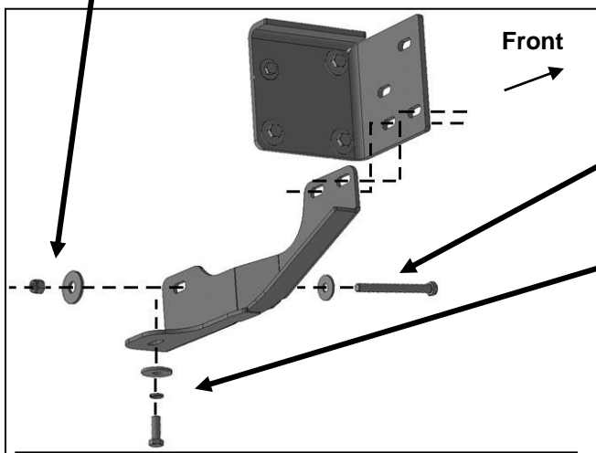
(Fig 9) Attach driver/left Support Bracket to bottom of frame extension and Frame Bracket
