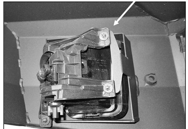
(Fig 14) Attach factory fog light assembly (if equipped) to mounting brackets on back of Bumper
