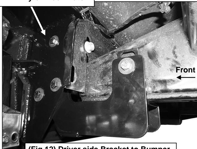
(Fig 12) Driver side Bracket to Bumper
