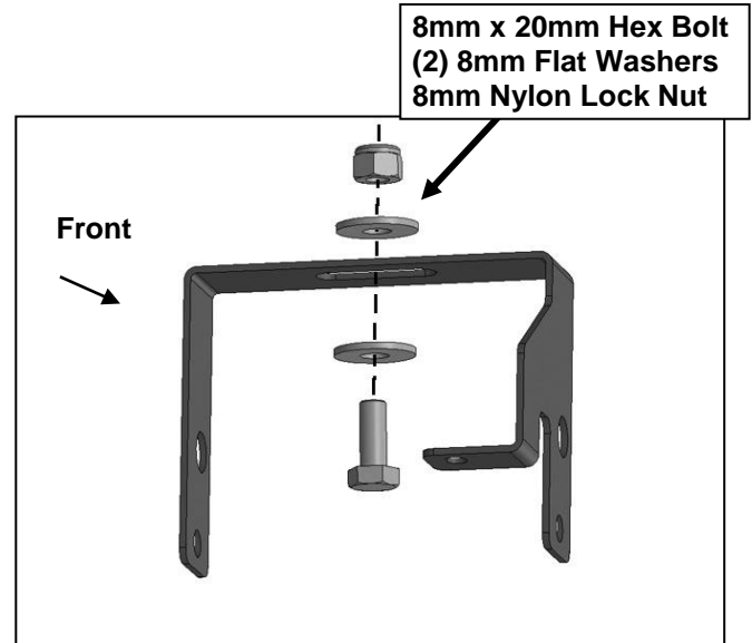
(Fig 16) Optional OEM fog light installation (light not included). Attach driver/left Upper Bracket to the slot in top of the opening
