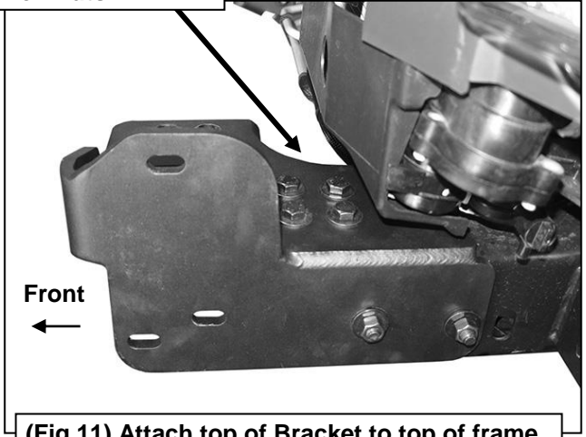
(Fig 11) Attach top of Bracket to top of frame
