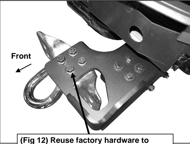
(Fig 12) Reuse factory hardware to attach tow hook to mount on Bracket
