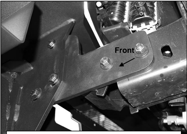
(Fig 14) Attach Bumper to side of Bracket (driver/left side pictured from behind bumper)
