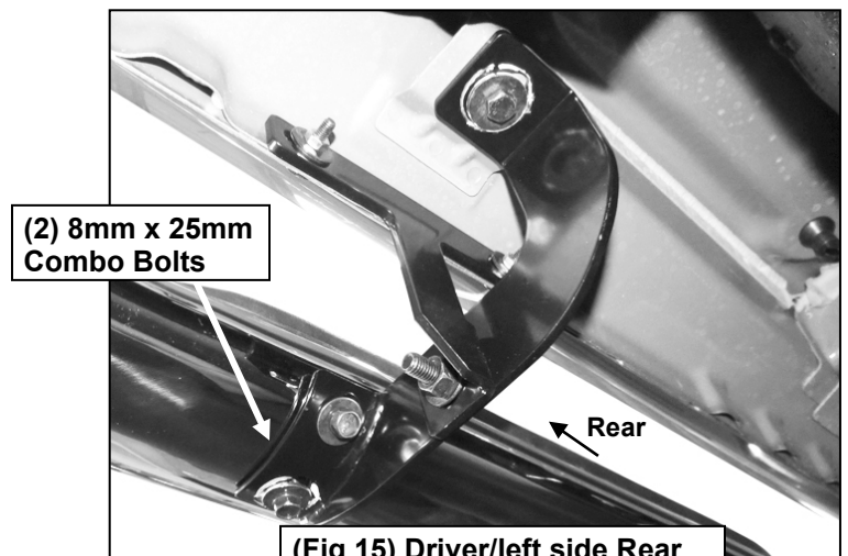
(Fig 15) Driver/left side Rear Brackets attached to Sidebar
