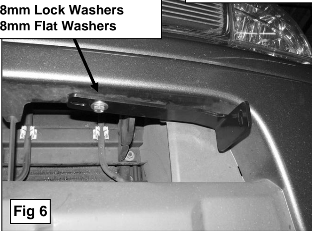
05-08 driver side Top Bracket installation pictured
