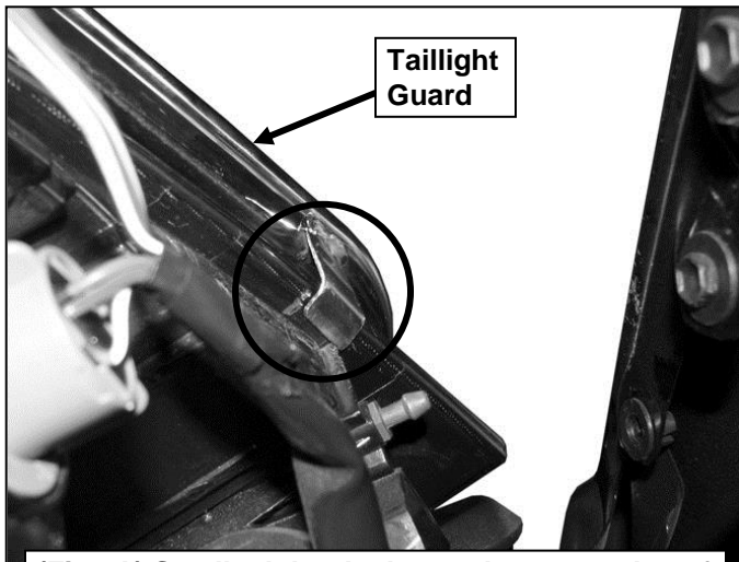
(Fig 4A) Small tab hooked onto the outer edge of the taillight assembly (back of taillight assembly pictured from above)
