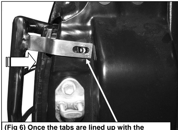
(Fig 6) Once the tabs are lined up with the mounting holes, push only the taillight assembly into place until the mounting pins "pop." DO NOT PUSH the taillight assembly all of the way in until the tabs on the Taillight Guard are lined up with the mounting holes
