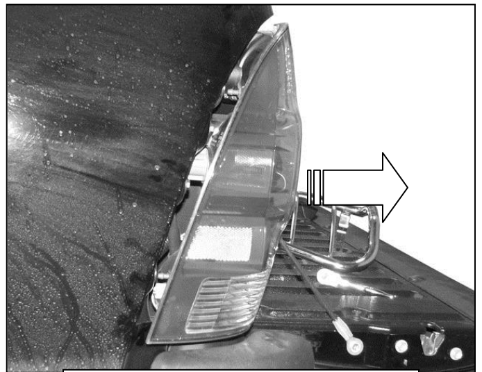
(Fig 2) Firmly grasp taillight assembly at top and bottom and pull straight out from vehicle (toward rear)
