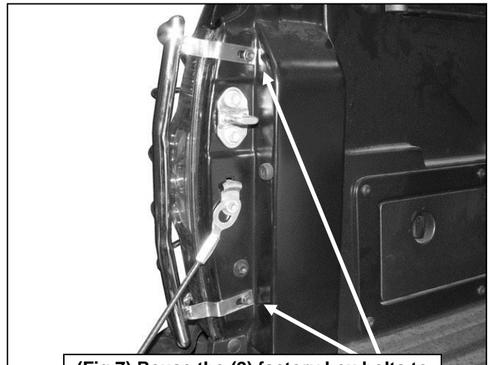
(Fig 7) Reuse the (2) factory hex bolts to attach the Taillight Guard to the vehicle
