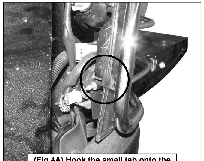
(Fig 4A) Hook the small tab onto the outer edge of the taillight assembly
