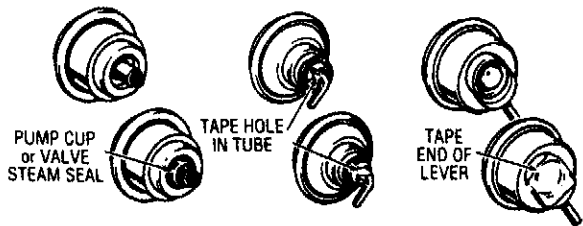
FIG. 3 VACUUM BREAK ADJUSTMENT INFORMATION PLUGGING AIR BLEED HOLES
