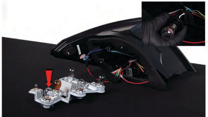
8) Remove the reverse bulb from the bulb plate. Transfer the bulb to the black and white wire reverse lamp socket of the Spyder tail light. Reinstall the socket.
