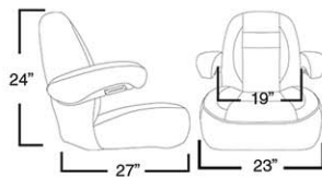
Seat Dimensions
