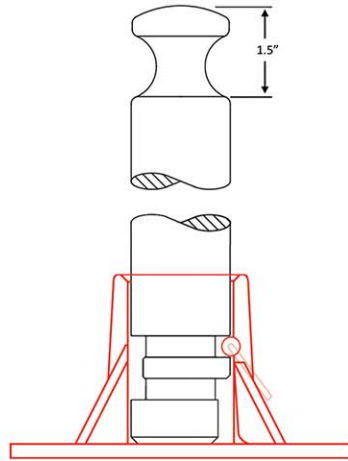
Notched in two points allowing easy drop-in and removal without accessing below the deck.
