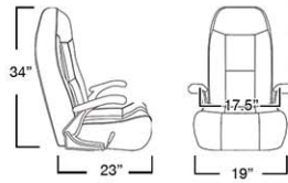
Seat Dimensions
