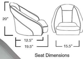
Seat Dimensions
