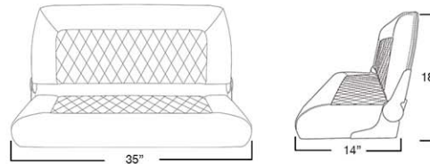
Seat Dimensions
