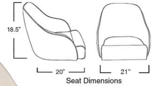
Seat Dimensions
