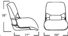
Seat Dimensions
