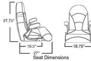
Seat Dimensions
