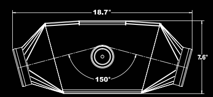
#9854 4" ULTRA LOW 150° ANGLE
