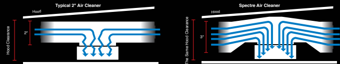
Drop base air cleaner assembly means increased filter area for increased airflow with the same hood clearance.
