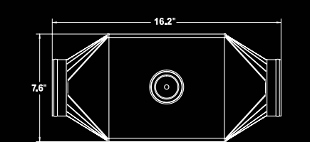
#9804 4" ULTRA LOW 180° ANGLE
