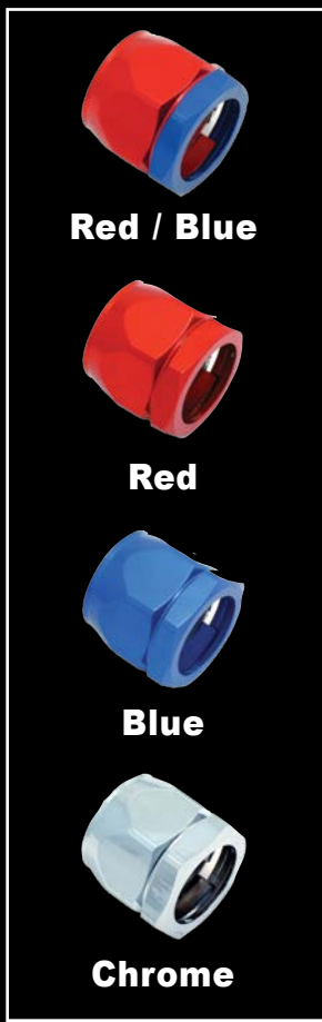
1-1/16" Inside Dia. Hose (#20 AN) 1-19/32" (1.6") Max Hose O.D. Including braid
