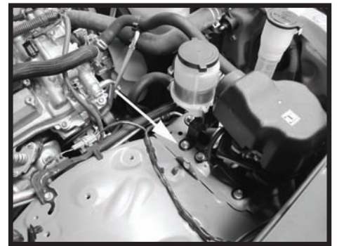
Step 13 Remove the bolt that secures the power steering reservoir. This bolt will be re installed with the new heat shield.
