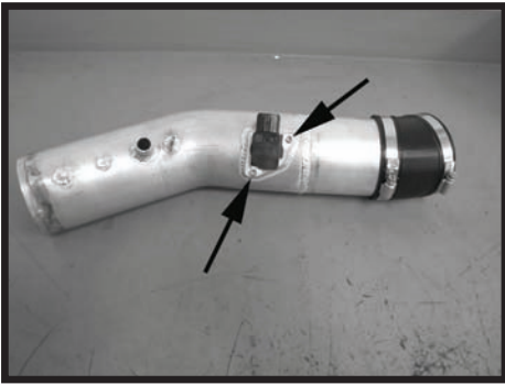
Step 11 Install the mass air flow sensor on the intake tube and secure with the supplied screws. Install the coupler on the end of the tube.
