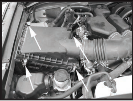
Step 8 Loosen the three bolts and remove the lower air box from the vehicle.
