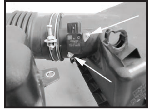
Step 10 Remove the MAFS from the factory air box.
