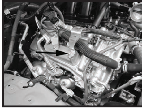
Step 9 Loosen the bolt that secures the factory intake tube mounting bracket and remove the bracket from the vehicle.
