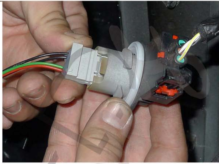
6. Connect the brake light harness to the LED taillight
