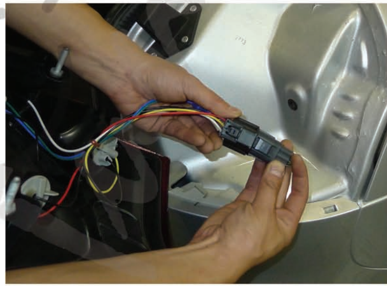
8. Connect the taillight harness to the LED taillight Please see the "L. E. D. tail lights installation instructions" If your tail lights don't have L. E. D. you can skip the installation instructions.
