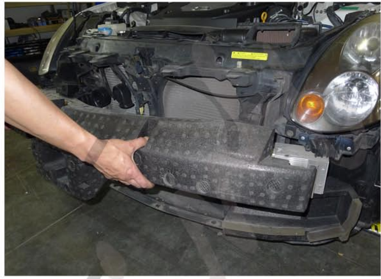
12. Remove the energy absorber
