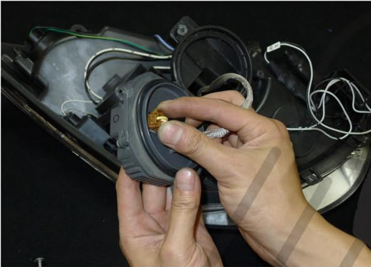
31. Connect the HID socket harness to the ballast
