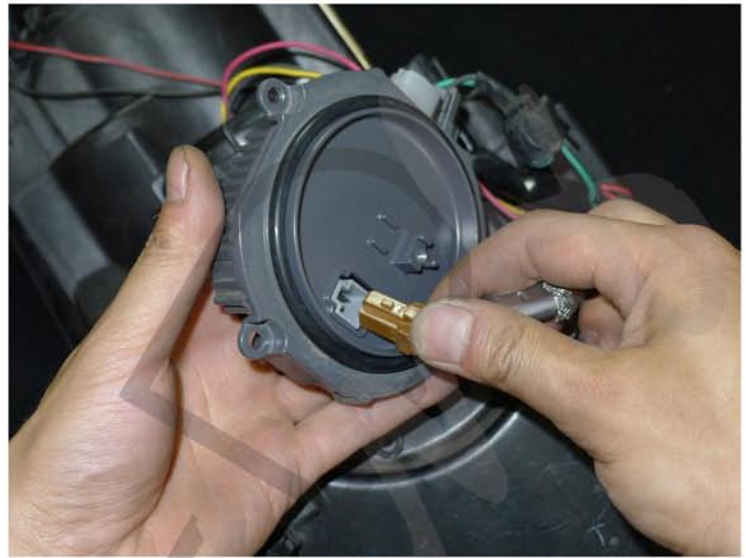
24. Disconnect the harness from the ballast
