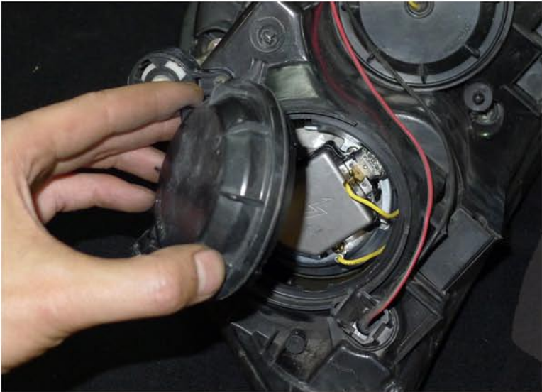
25. Remove the HID bulb to access the hole cover
