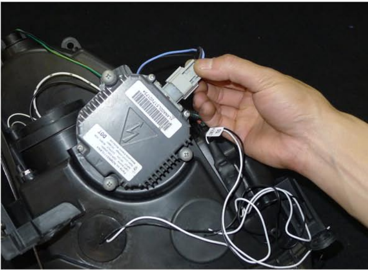
35. Connect the hadlight harness to the ballast Please see the "Halo and L.E.D installation instructions" If your headlights don't have HALO or L.E.D. You can skip this step
