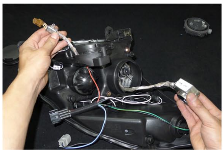
28. Run the HID socket harness through the new headlight housing
