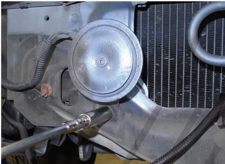
13. Loosen the 10mm bolt
