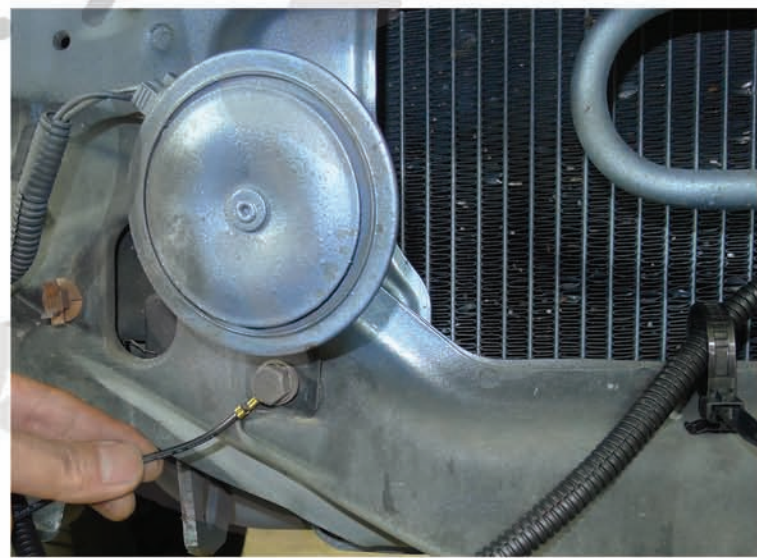
14. Place the fog light harness ground wire behind 10mm bolt
