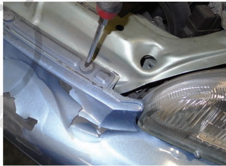
26. Tighten the (5) phillips head screws
