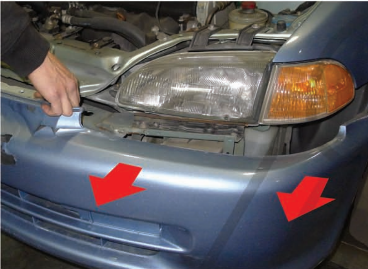
7. Remove the front bumper
