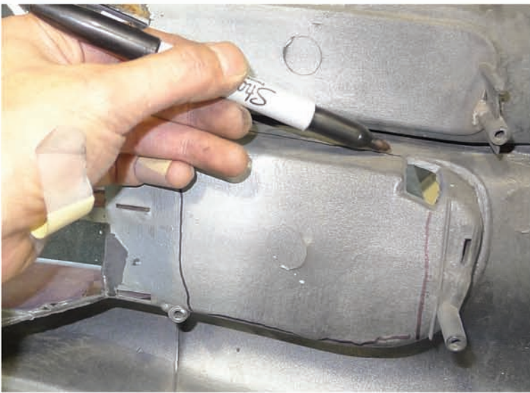
17. Mark the area to be cut with the marker
