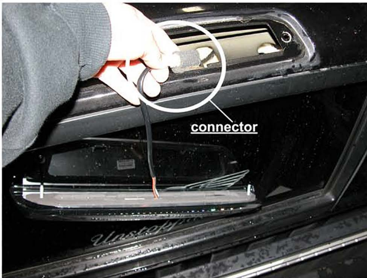
7. Plug the connector harness with the new 3rd brake light
