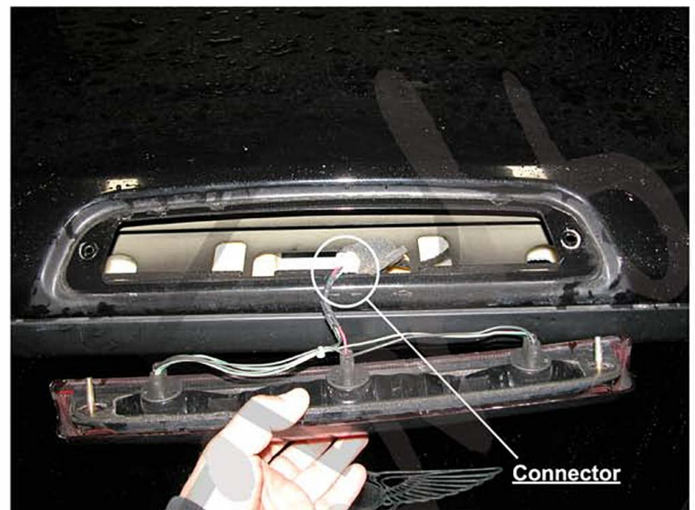
4. After you pull out the 3rd brake light, you will see all the wires and connector harnesses
