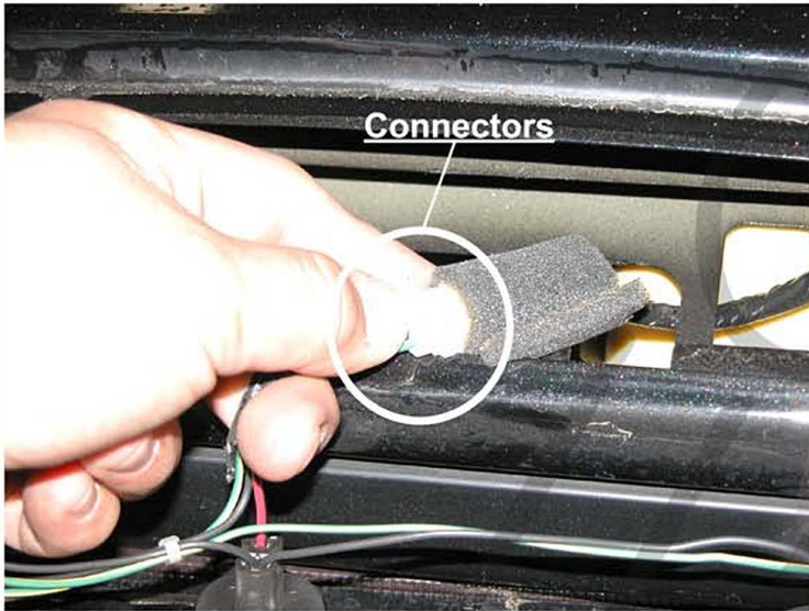
5. Disconnect the connector harness from the vehicle
