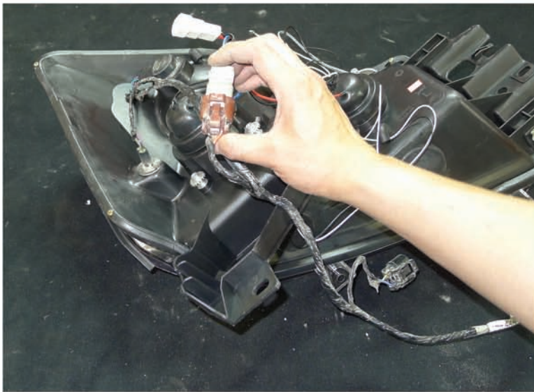
23. Connect the headlight sub-harness to the new projector headlight
