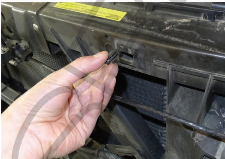
33. Remove the (4) plastic clips from the radiator support
