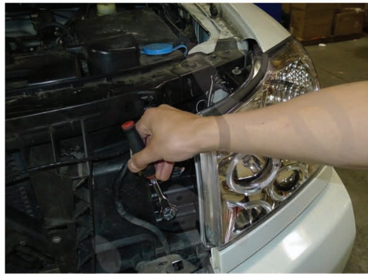
30. Tighten the 8mm bolt
