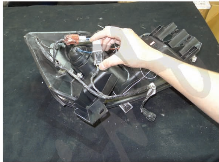
24. Connect the headlight sub-harness to the new projector headlight
