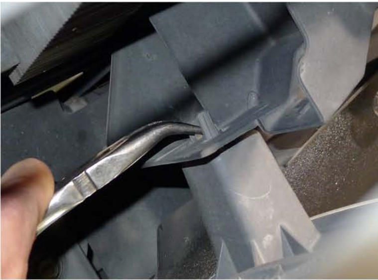
17. Release the (6 )grill mounting clips
